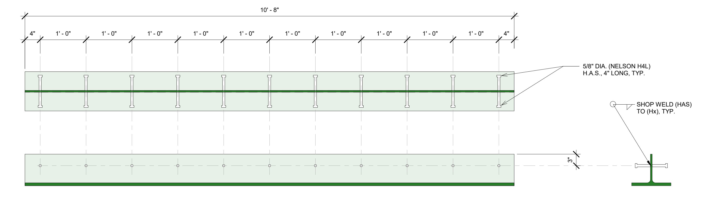
[H2] WT8x38.5 HEADER BEAMS OVER TRANSPORT OPENING SCALE: 1" = 1'-0"
