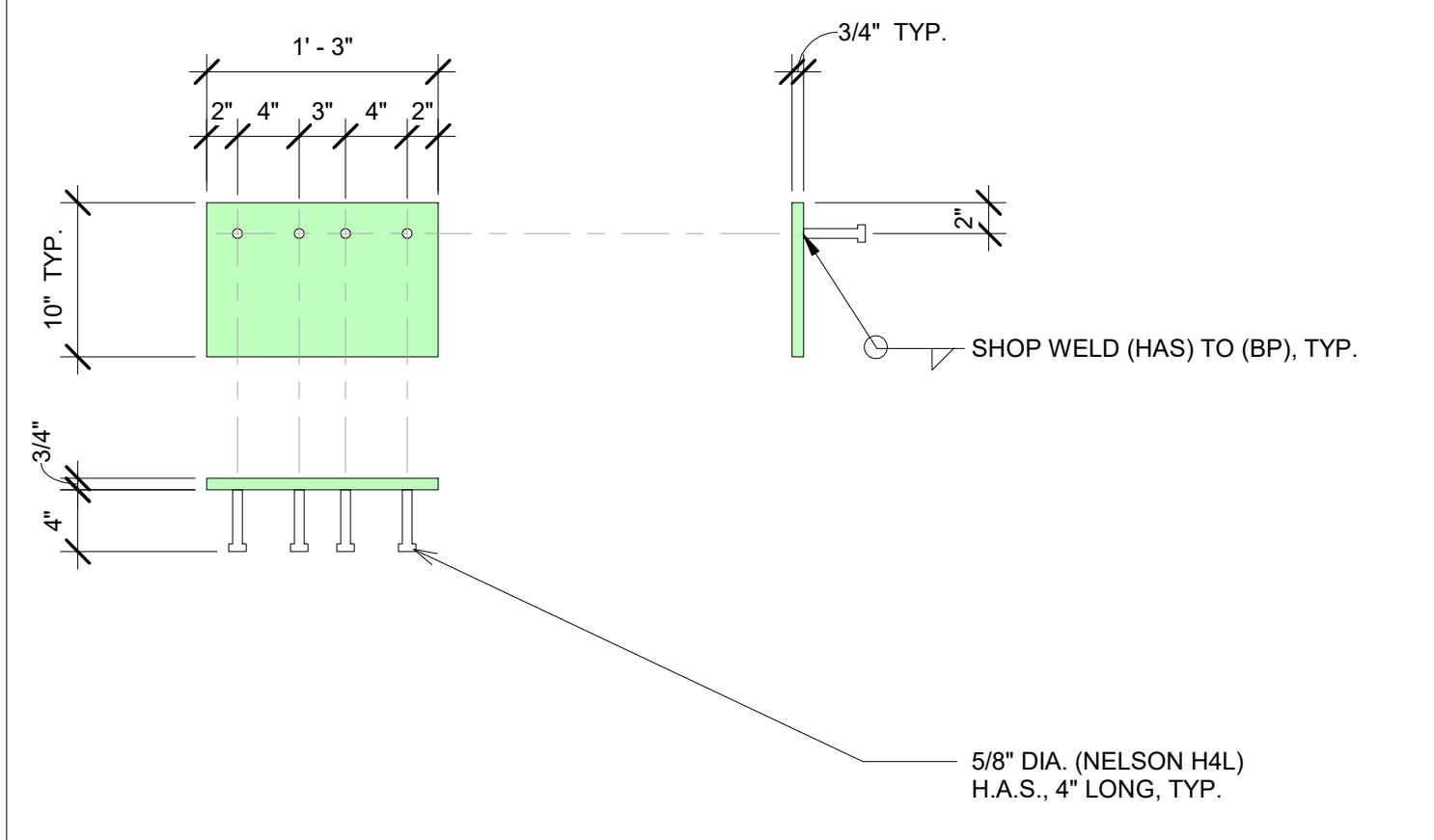
[BP10-15] 3/4" THICK BEARING PLATE SCALE: 1" = 1'-0"
