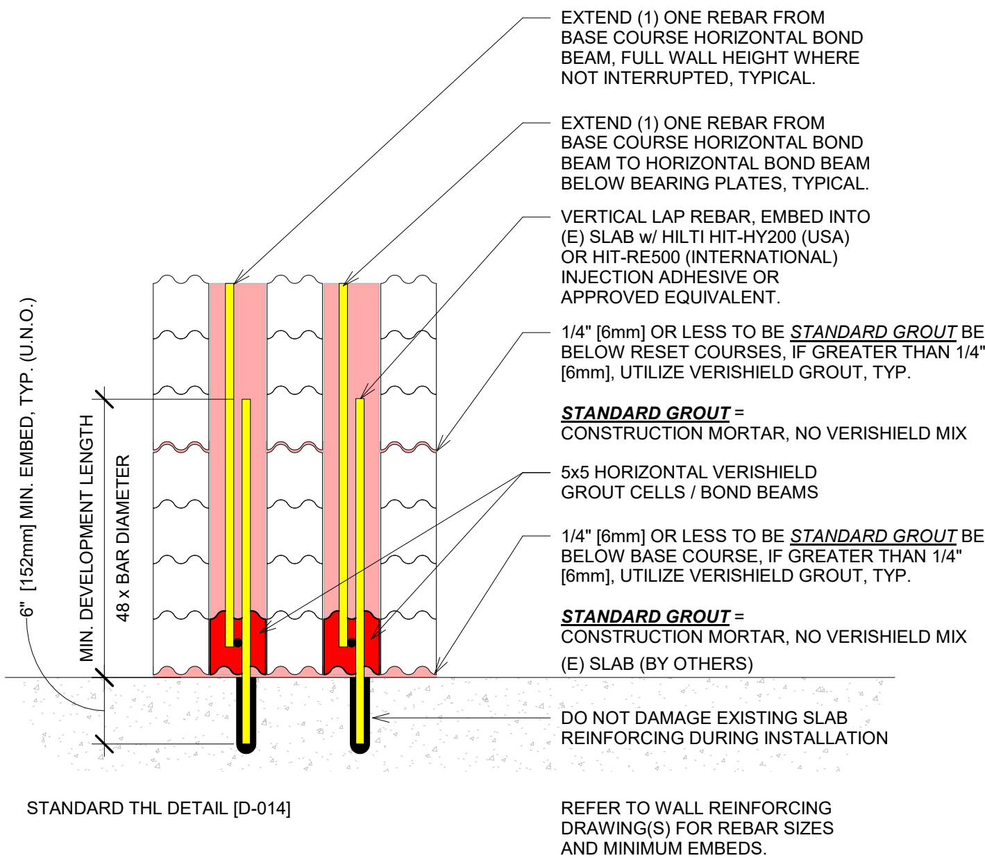
2 TYPICAL REBAR EMBED DETAIL 1" = 1'-0"
