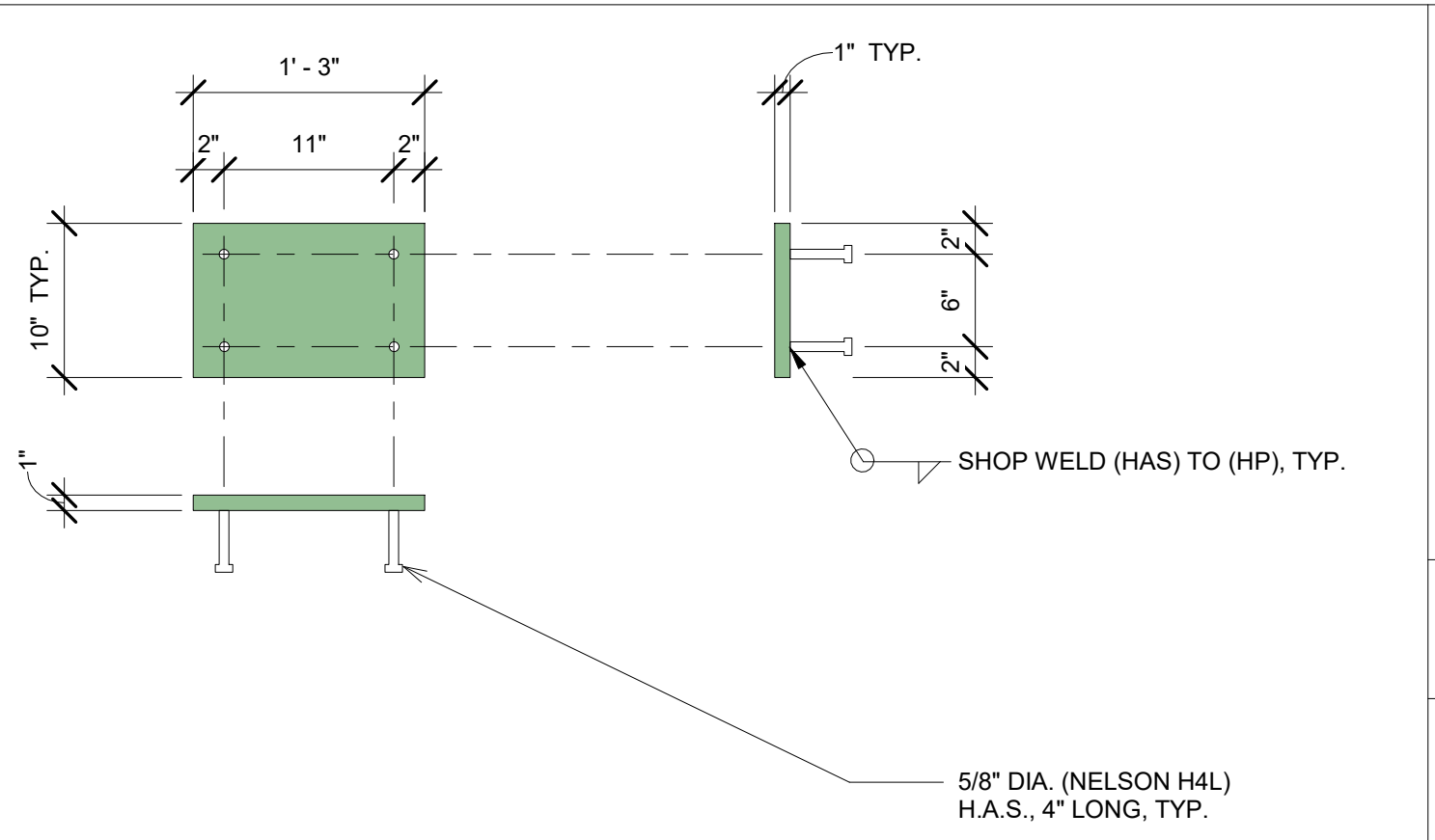
[HP10-15] 1" THICK HEADER PLATE SCALE: 1" = 1'-0"
