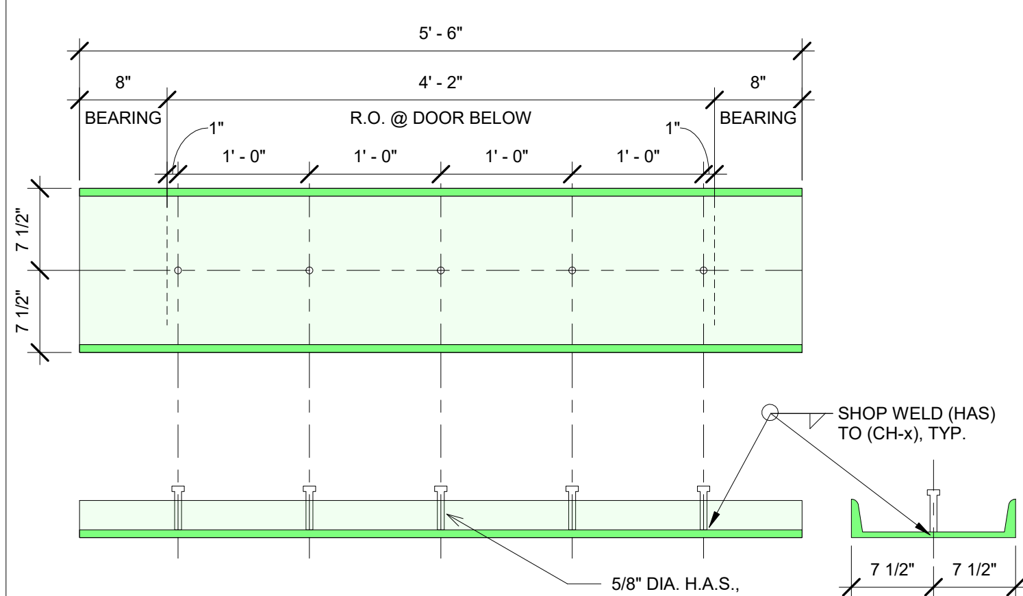
[CH-2] C10x30 CHANNEL - LOOSE LINTEL OVER DOOR OPENING SCALE: 1" = 1'-0"
