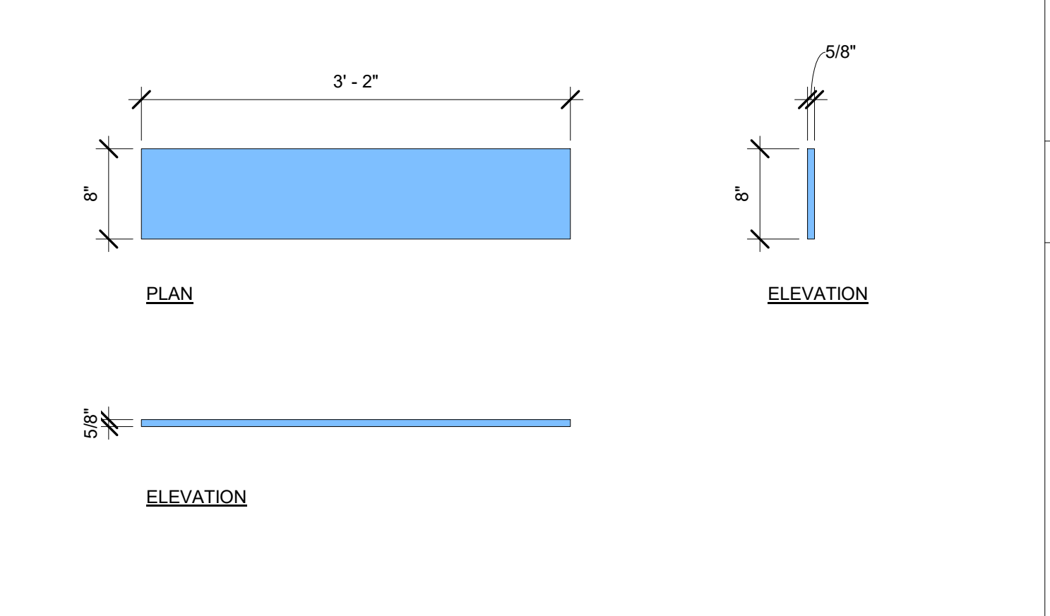
[DS-38] 5/8" THICK DIAPHRAGM STRAP SCALE: 1" = 1'-0"
