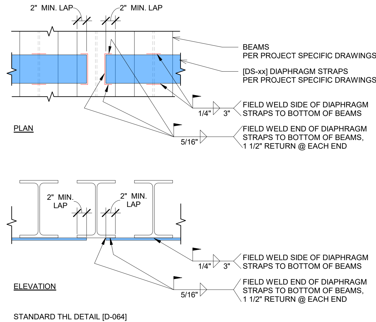
4 DIAPHRAGM STRAP TO BEAM DETAIL 1" = 1'-0"
