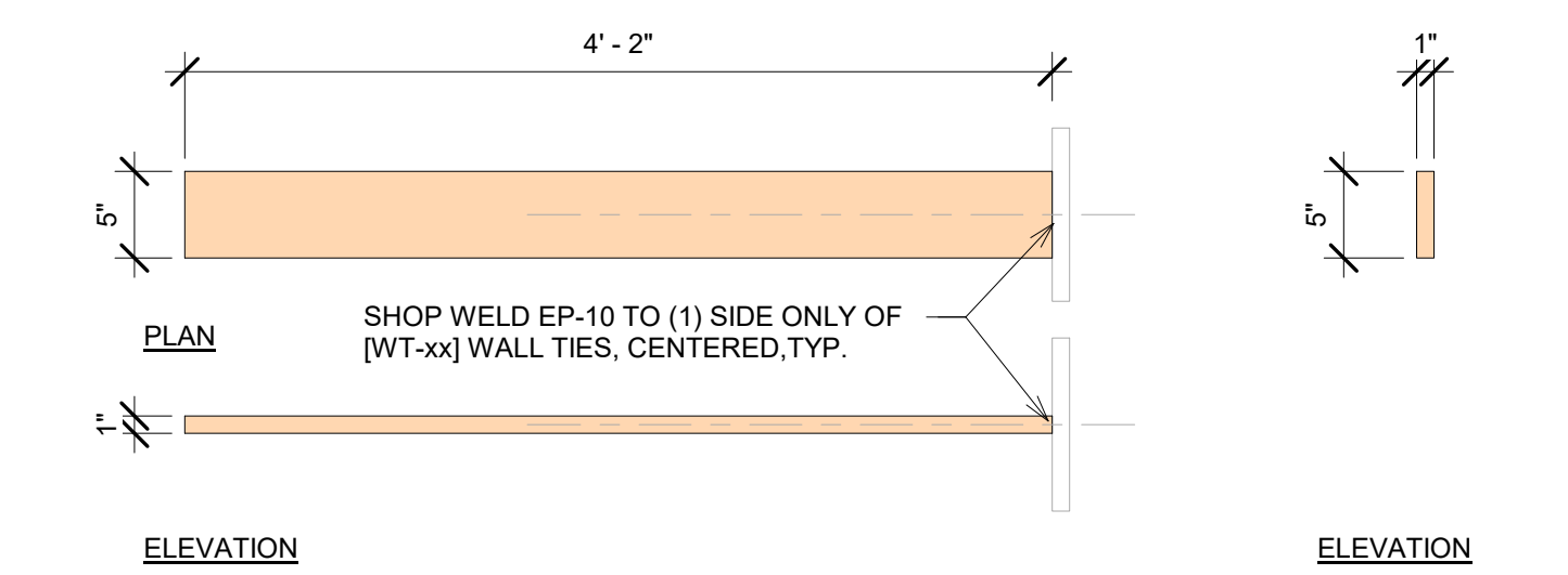
[WT-50] 1" THICK WALL TIE SCALE: 1" = 1'-0"
