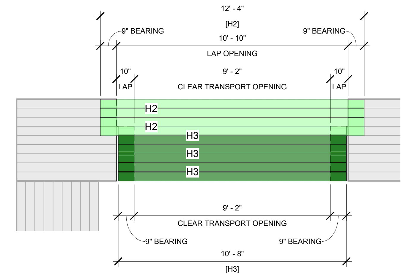
3 Headers Over Transport Opening 3/8" = 1'-0"
