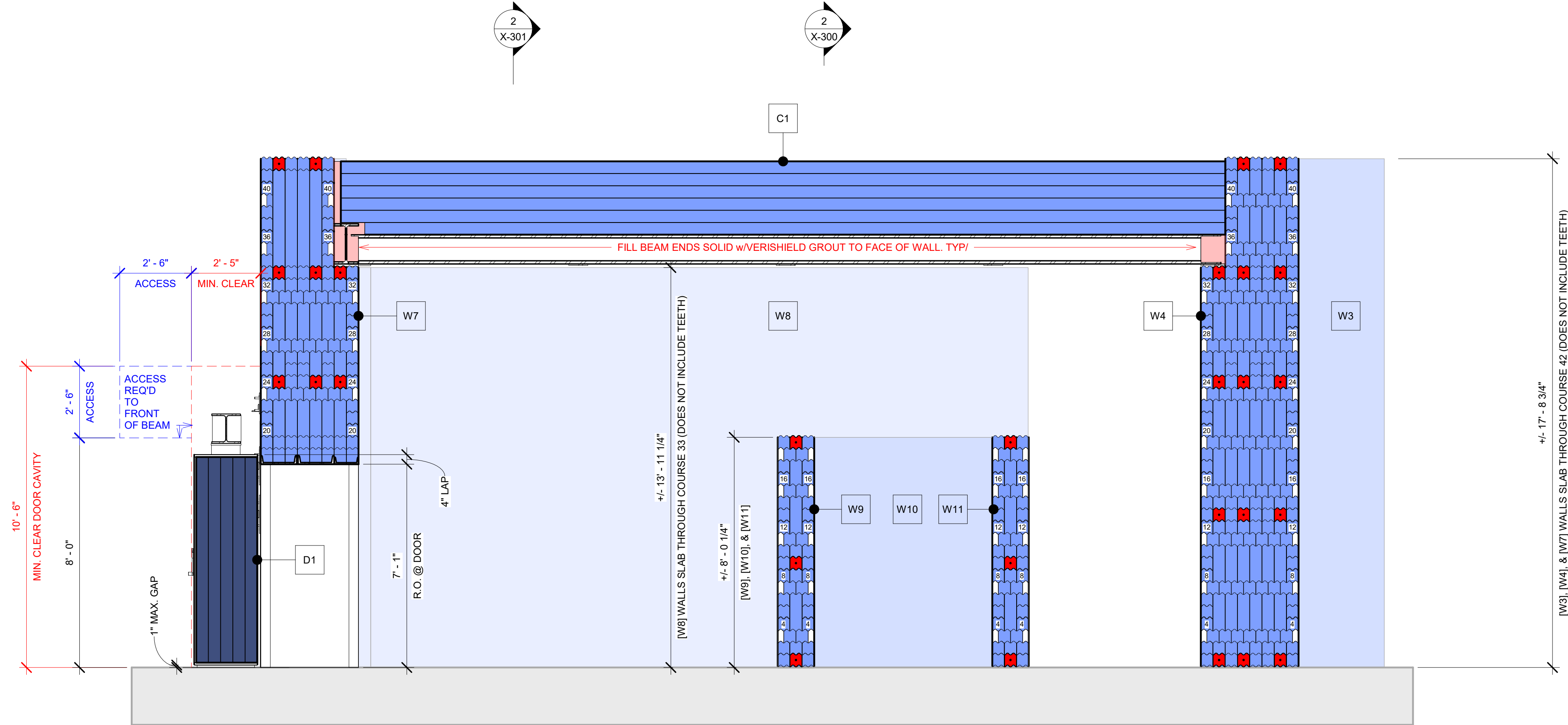
1 Section Through Door 3/8" = 1'-0"
