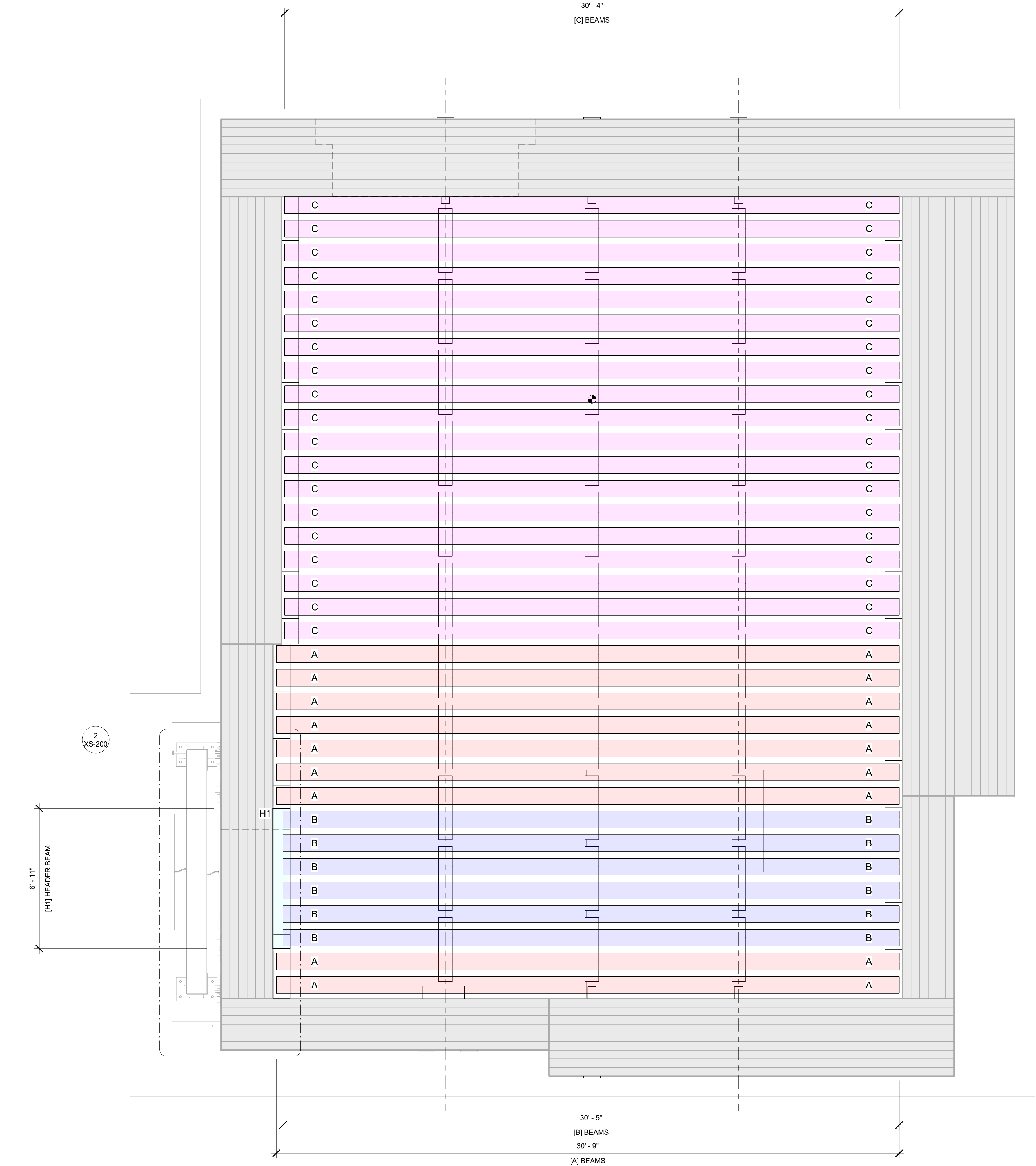
1 Framing Plan 3/8" = 1'-0"
