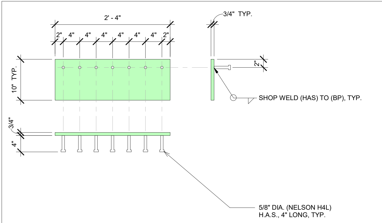
[BP10-28] 3/4" THICK BEARING PLATE SCALE: 1" = 1'-0"
