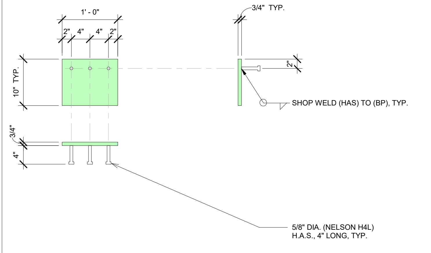
[BP10-12] 3/4" THICK BEARING PLATE SCALE: 1" = 1'-0"
