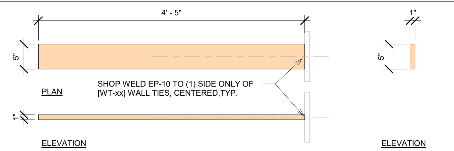
[WT-53] 1" THICK WALL TIE SCALE: 1" = 1'-0"
