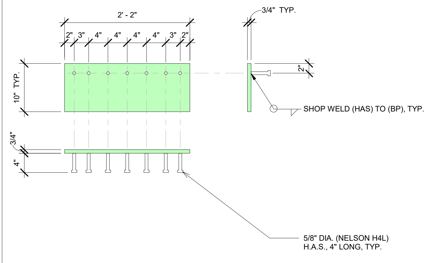
[BP10-26] 3/4" THICK BEARING PLATE SCALE: 1" = 1'-0"
