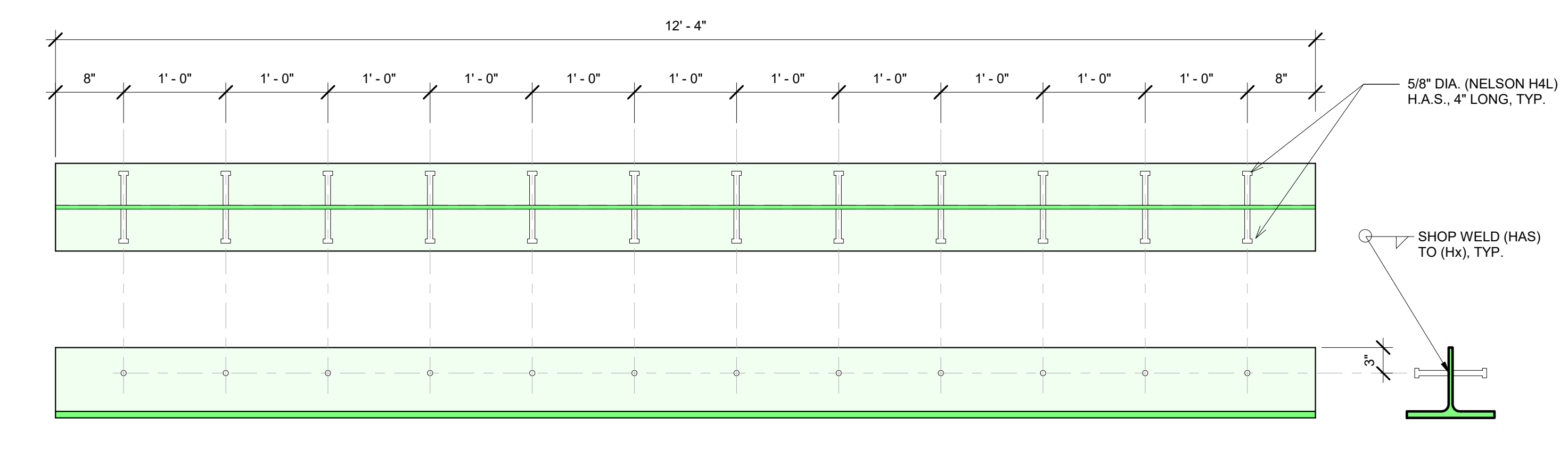
[WT-38] 1" THICK WALL TIE SCALE: 1" = 1'-0"
